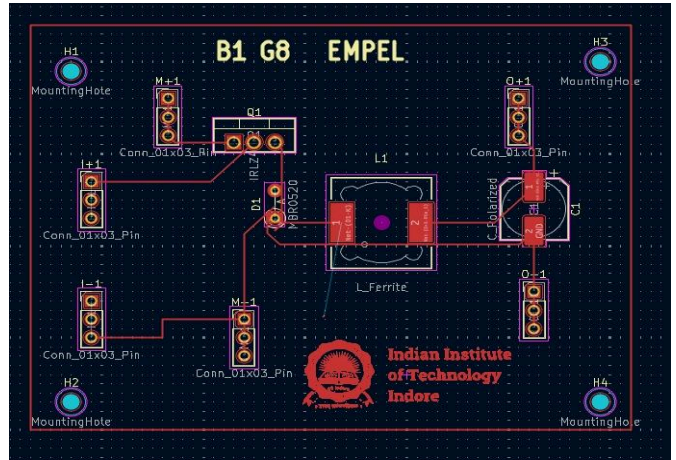
Converter PCB Layout
