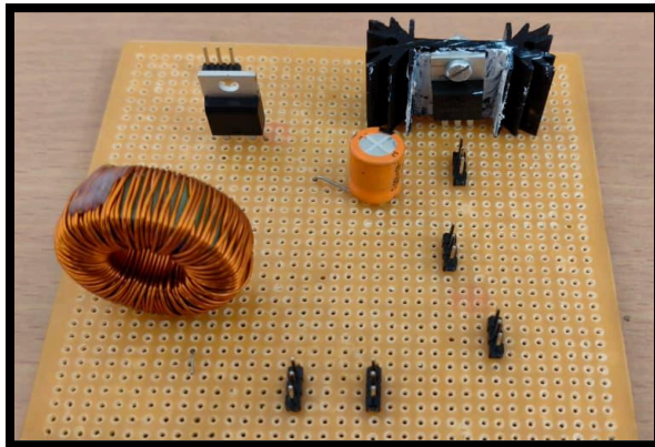
Soldered Buck Converter
