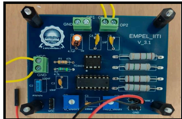
Gate Driver Circuit
