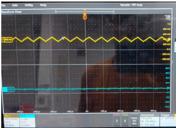
PWM (15KHz, 50% Duty Cycle)
